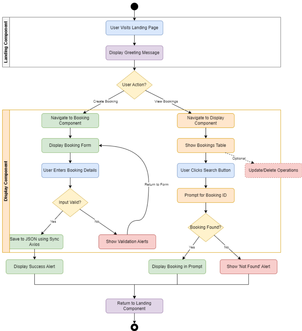
Travel Booking System - Activity Diagram
